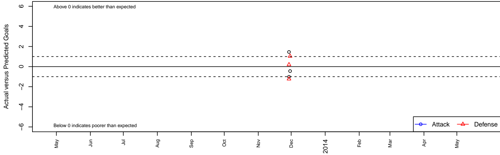
Matanuska AKFC 03 Aurora G02 Dots are actual minus expected GF (blue circles) and GA (red triangles). Blue line is smoothed change in attack strength. Red is smoothed change in defense strength.
